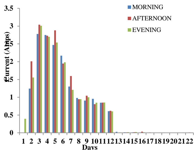
Fig. 3: Electric Current generation from sample obtained from Bola paunch, Akure
