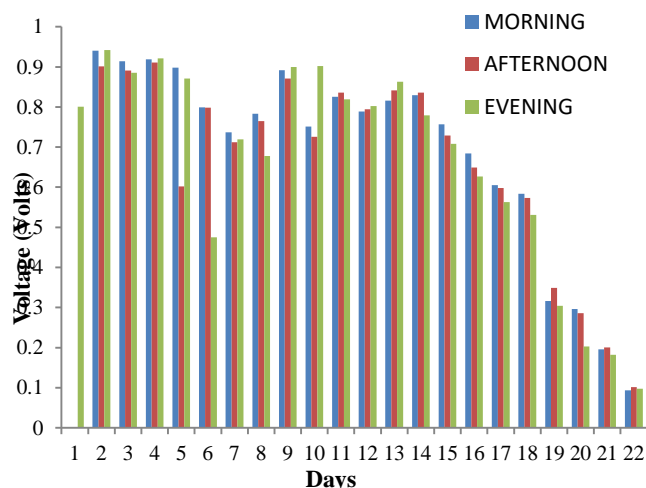
Fig. 4: Electric Voltage generation from sample obtained from Topland paunch, Akure
